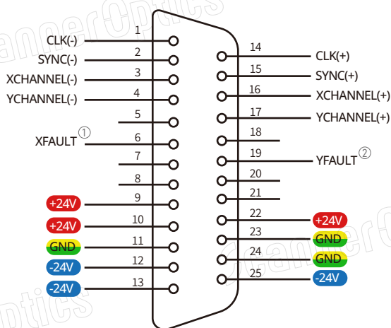
XY2-100通讯协议 Communication Protocol
